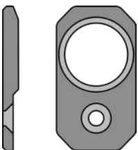
DP-94 Right FLIP-CHIP - The derailleur hanger and simultaneously a variable frame component for Esker RS, allowing for geometry adjustments.
